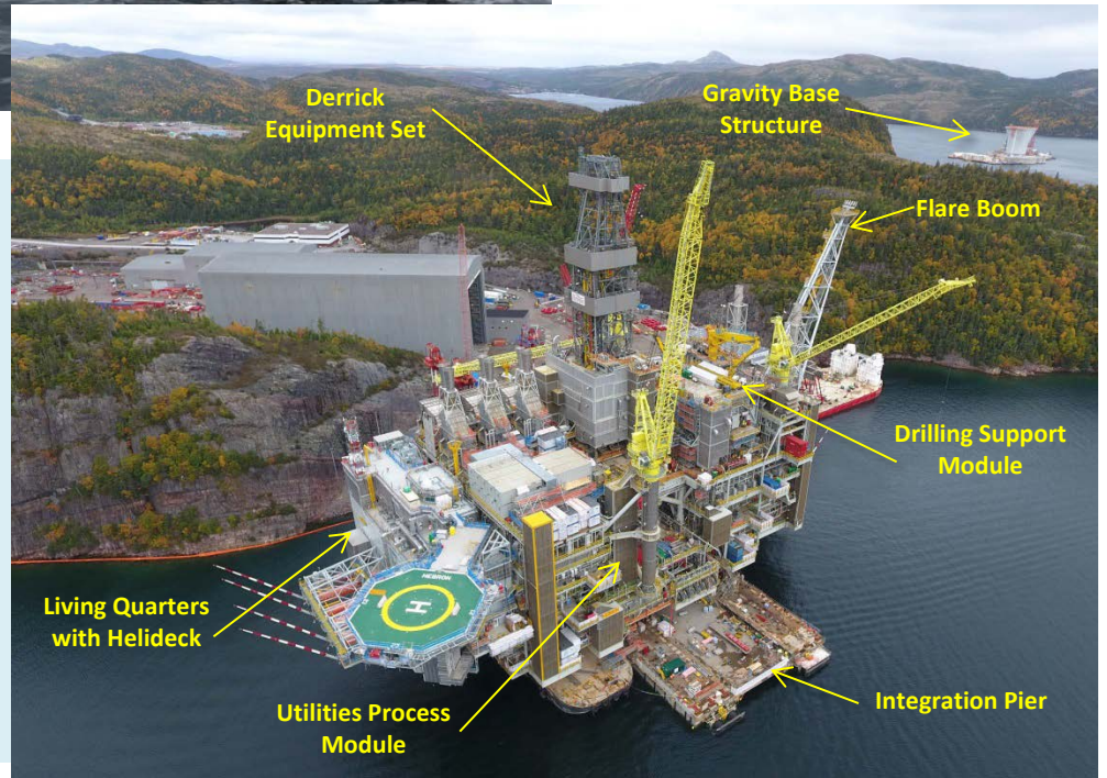
The integrated Topsides modules sit on the Bull Arm integration pier.
