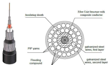
Figure 6 – Double Armoured Cable (DA)
