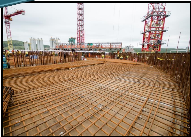
Rebar installation on GBS storage cells and ice walls in preparation for roof pour
